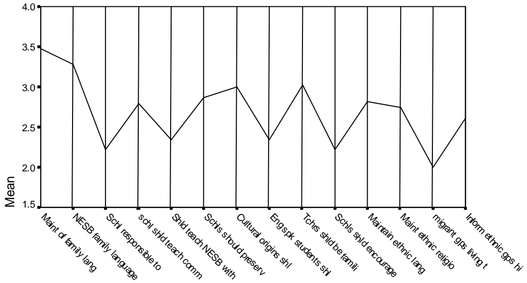
Comparison of means across 14 multicultural questions
